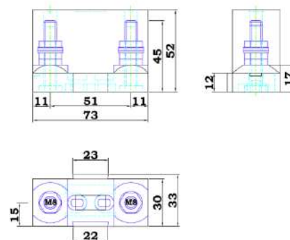
CIP100200100 = Modular fuse holder for Mega-fuse
